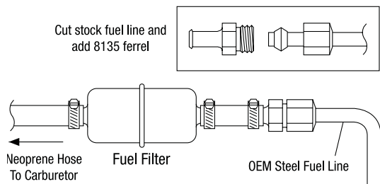
Fig. 3 - Fuel Line Kit #8135 Installed on Stock Steel Line
